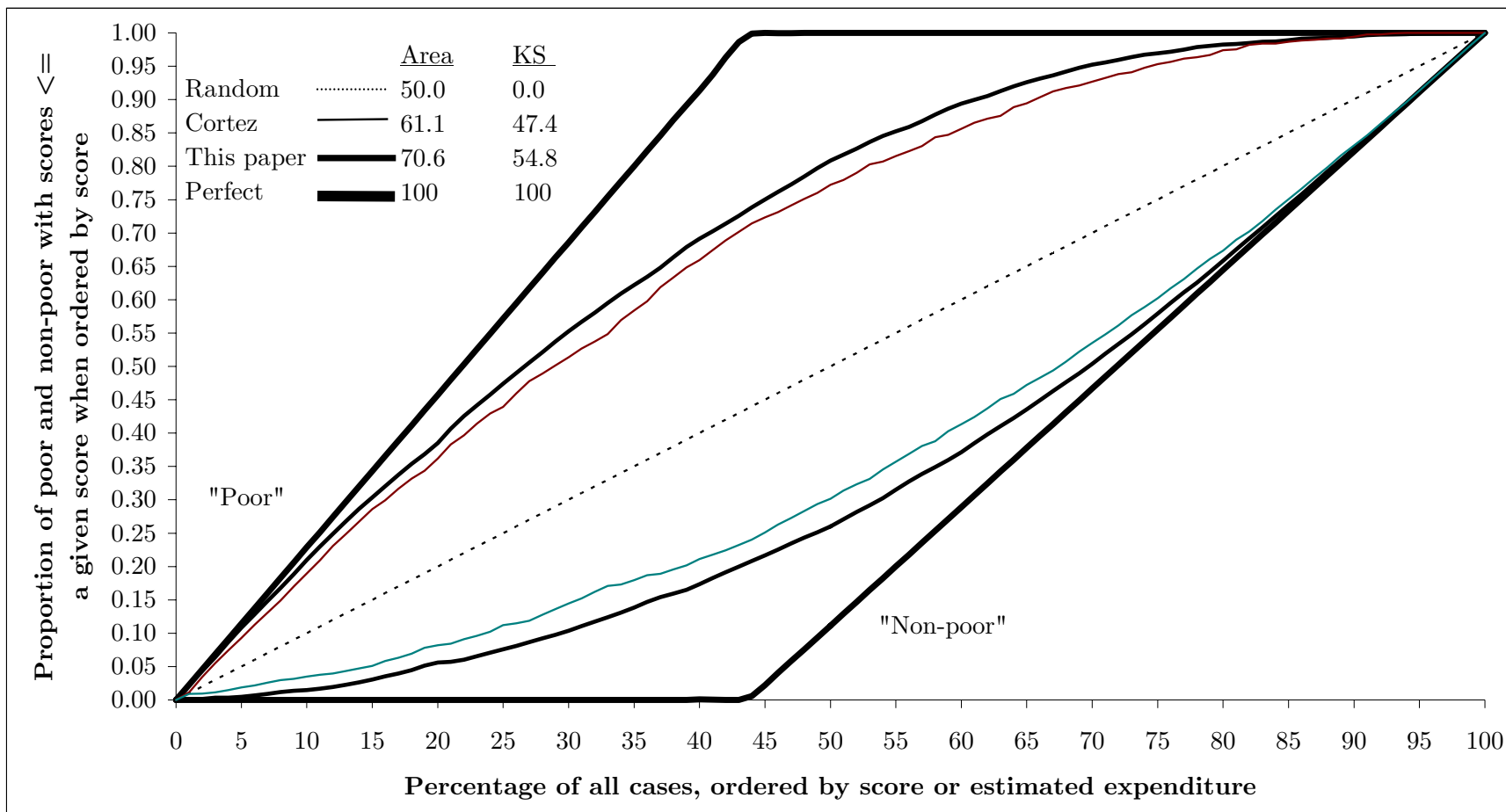
Figure 14: Targeting accuracy as measured by ROC curves, Bangladesh poverty scorecard from Cortez et al. (2005) and from this paper
